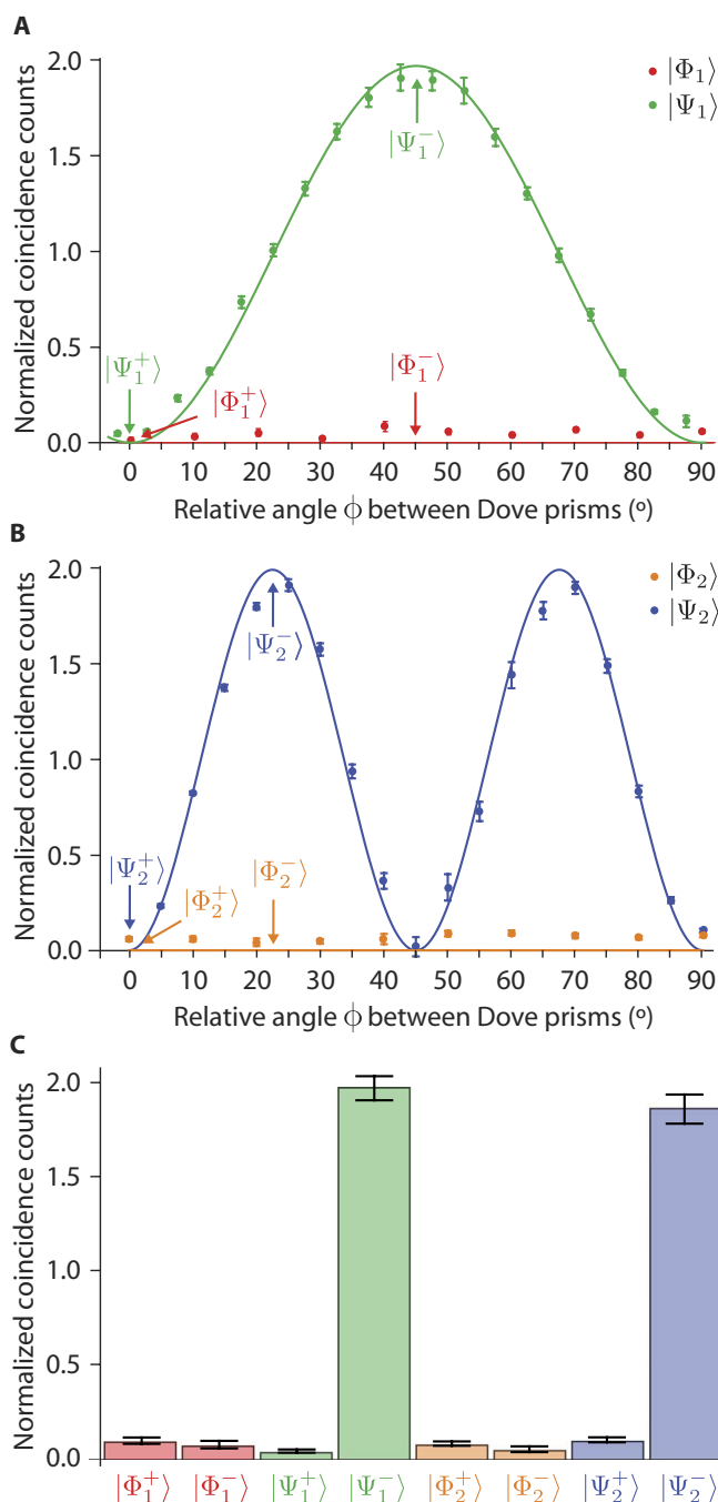
Fig. 3. Coincidence counts as a function of input state. (A) Graph showing the variation of coincidence counts for the input states |\Psi_1\rangle , indicated by the green points, and |\Phi_1\rangle , indicated by the red points. The theoretical variation in coincidence counts of any |\Psi_1\rangle input state is equal to 2 \sin^2(2\phi) . For any |\Phi_1\rangle input state, the coincidence counts should remain zero as a function of \phi . The normalized count rate is determined by dividing the coincidence rate in the dip/peak by that outside of the dip/peak. The error bars represent 1 SD from averaging 20 readings. (B) Graph showing the variation of coincidence counts for the input states |\Psi_2\rangle , indicated by the blue points, and |\Phi_2\rangle , indicated by the orange points. The theoretical variation in coincidence counts of any |\Psi_2\rangle input state is equal to 2 \sin^2(4\phi) . (C) Normalized coincidence counts for the OAM \ell = 1 and 2 Bell states. Only the |\Psi_1^+\rangle and |\Psi_2^-\rangle input states result in coincidences being recorded.
